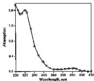
UV9380C UV Absorption Spectrun 0004 N in Methylene chloride
